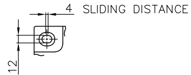
FRAME FOOT AS VIEWED FROM BELOW
