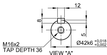
VIEW "A"
