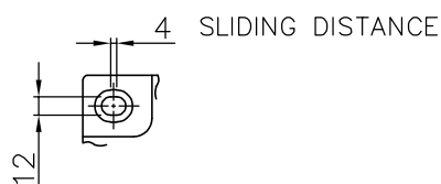
FRAME FOOT AS VIEWED FROM BELOW
