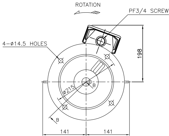
BOTTOM VIEW OF SHAFT END
