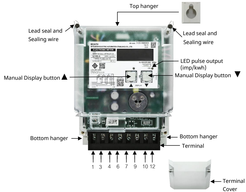
Figure 2.1 The parts of meter
